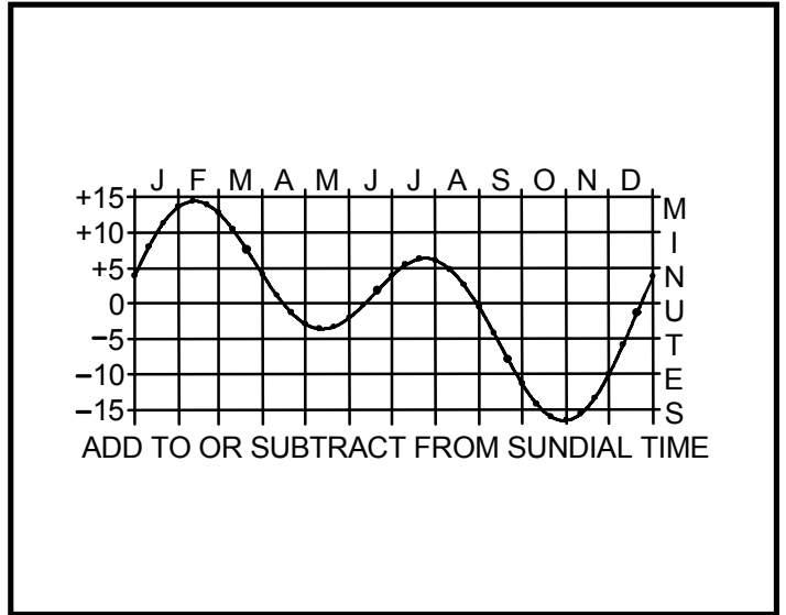
Equation of Time Graph
